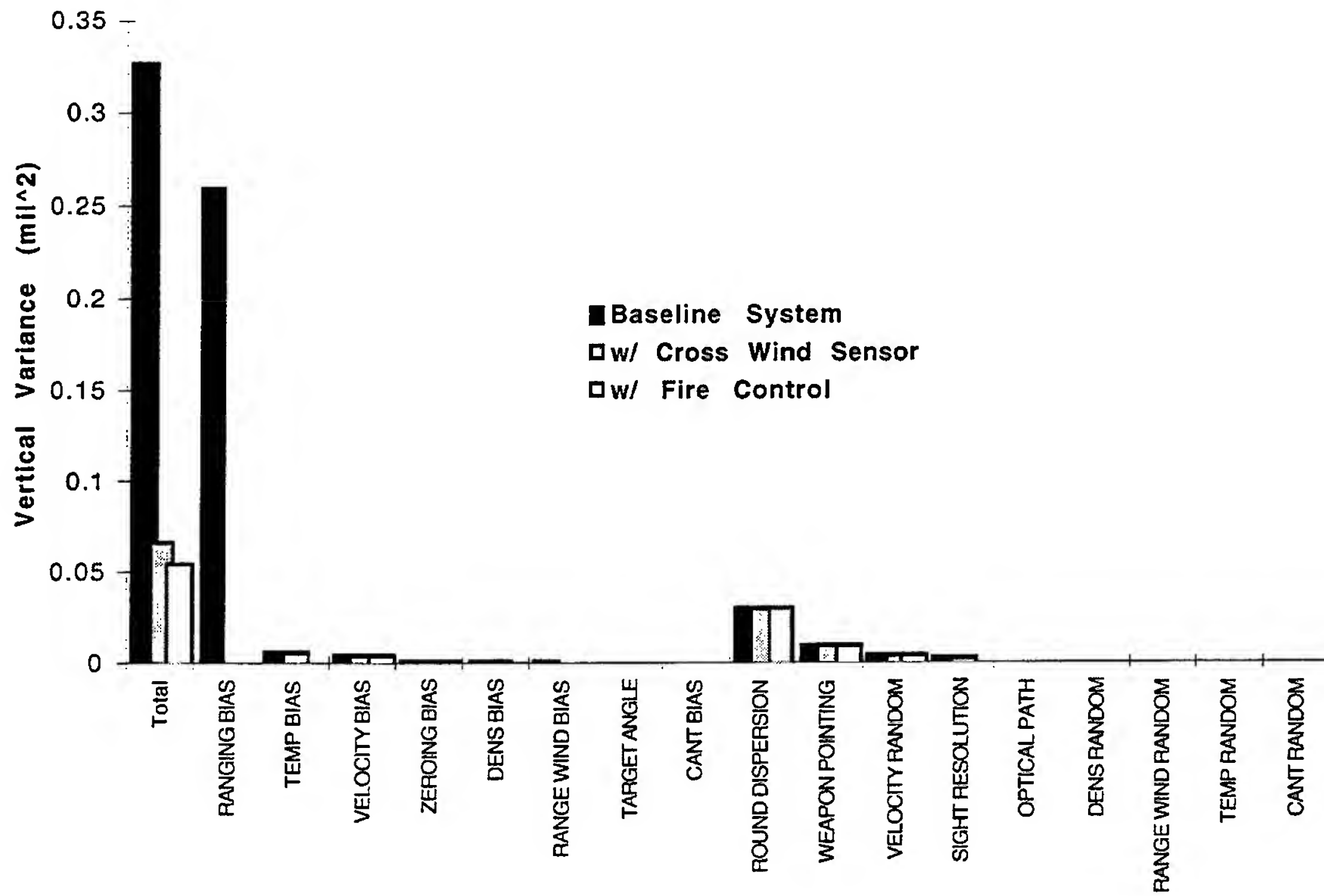
Figure 7. Vertical Variances, 300 WM, 700 m.
